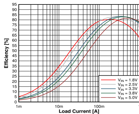
图 9-5. Efficiency
