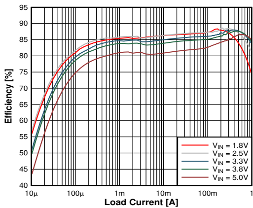
图 9-2. Efficiency
