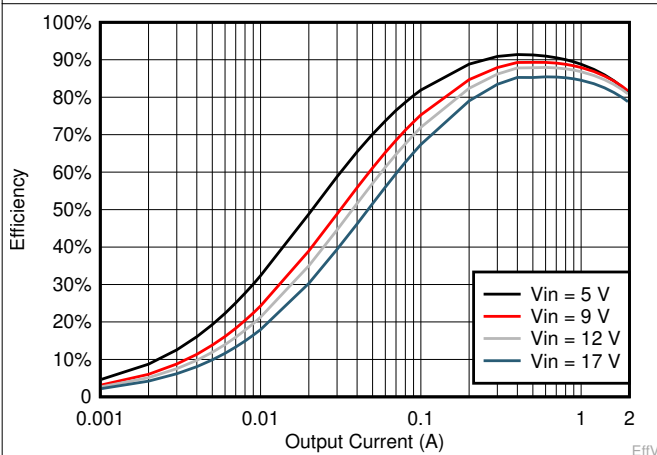
图 7-11. V_{OUT} = 1.5\text{ V} Efficiency, L = 2.2\text{ }\mu\text{H}
