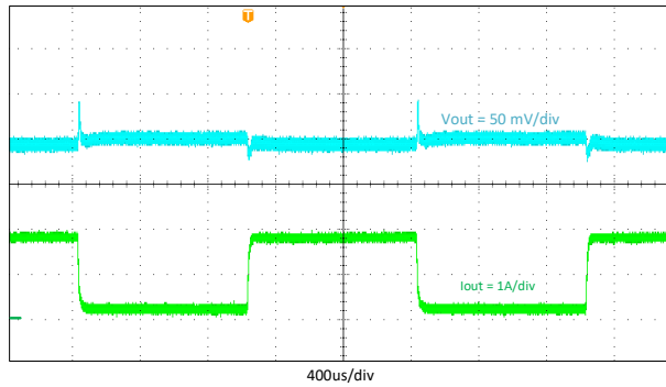
图 9-8. Transient Response, 0.2 to 1.8 A
