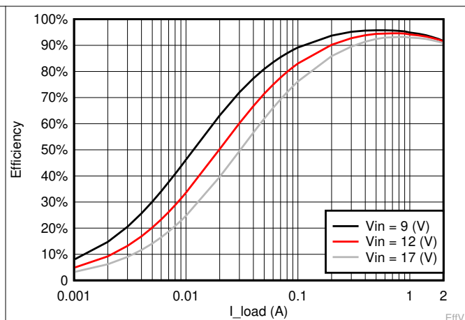
图 7-14. V_{OUT} = 5 V Efficiency, L = 4.7 \mu H
