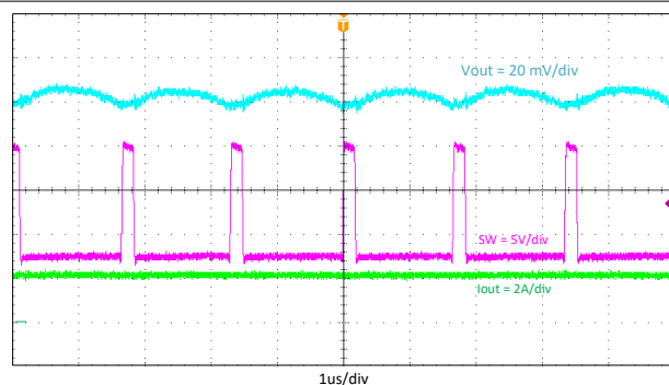
图 9-6. Output Voltage Ripple, I_{out} = 2\text{ A}
