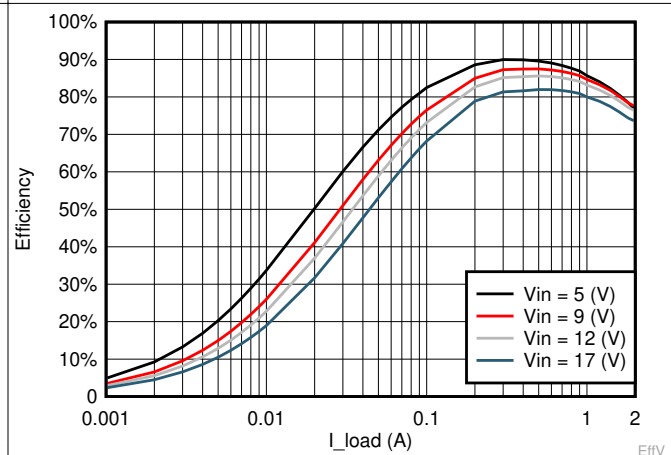
图 7-10. V_{OUT} = 1.05\text{ V} Efficiency, L = 2.2\text{ }\mu\text{H}
