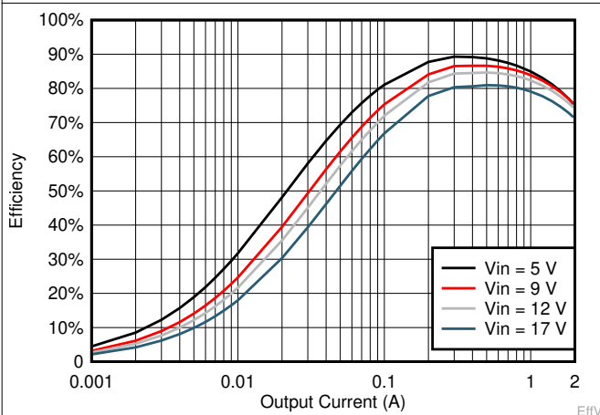
图 7-9. V_{OUT} = 0.95\text{ V} Efficiency, L = 2.2\text{ }\mu\text{H}
