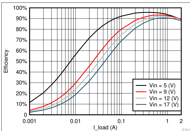
图 7-13. V_{OUT} = 3.3 V Efficiency, L = 3.3 \mu H
