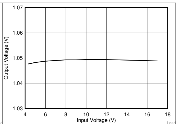
图 9-3. Load Regulation with Different Input Voltage
