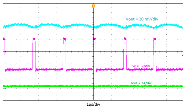
图 9-5. Output Voltage Ripple, I_{out} = 0.2\text{ A}
