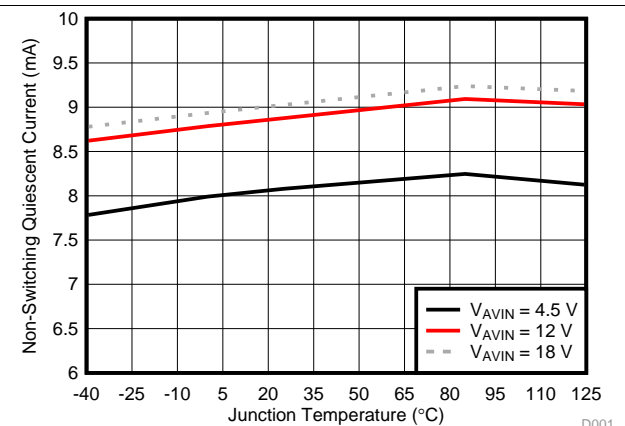
图 9. Non-Switching Input Current ( I_{AVIN} ) vs Junction Temperature
