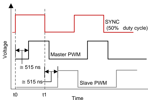
图 28. Phase Interleaving Timing
