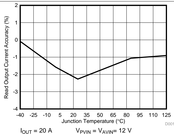
图 15. READ_IOUT Accuracy vs Junction Temperature
