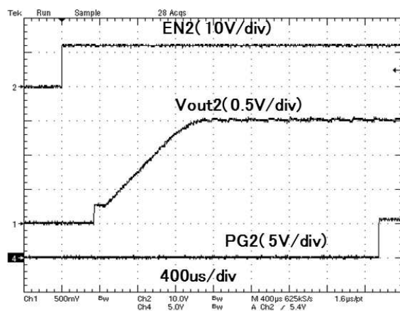
Figure 11. V_{O2}=1.5\text{V} , PG
