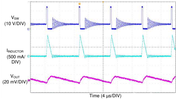
图 25. LM76005 Switching Waveform and Output Ripple
