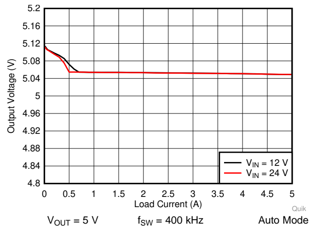
图 19. LM76005 Load and Line Regulation
