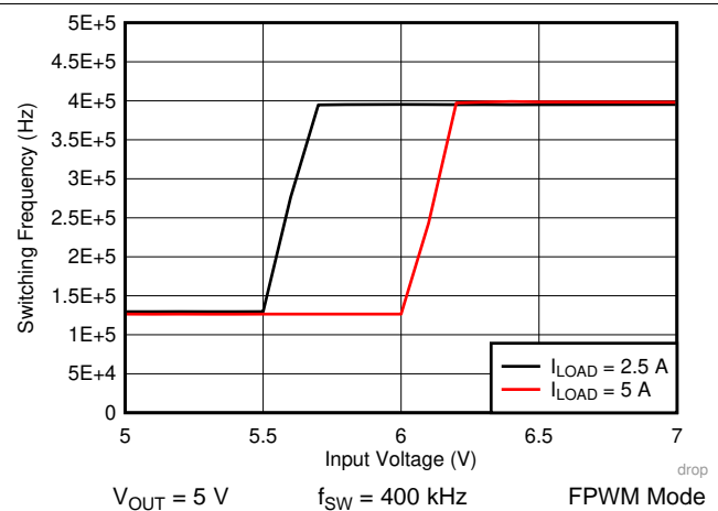
图 21. LM76005 Frequency Dropout
