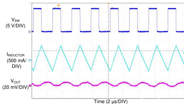
图 26. LM76005 Switching Waveform and Output Ripple
