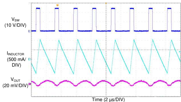
图 27. LM76005 Switching Waveform and Output Ripple
