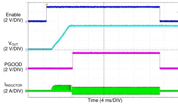
图 30. LM76005 Start-up Waveform
