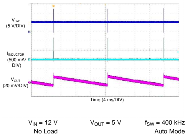
图 22. LM76005 Switching Waveform and Output Ripple
