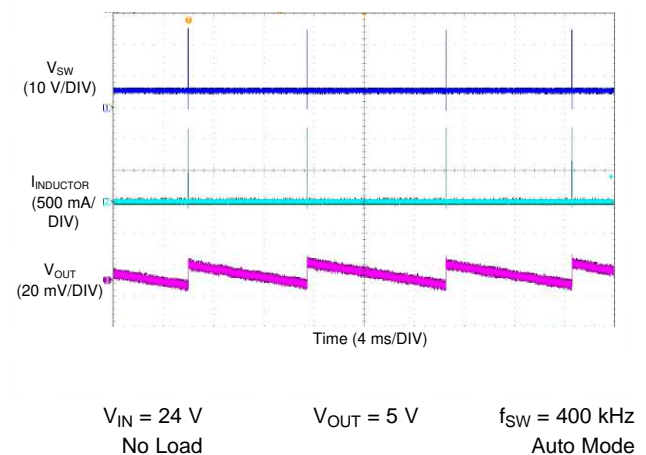
图 23. LM76005 Switching Waveform and Output Ripple
