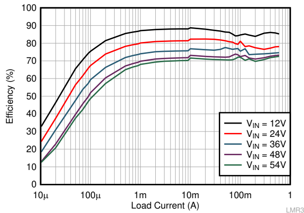
LMR36506R3 V_{OUT} = 3.3 V Fixed 1 MHz (AUTO)
