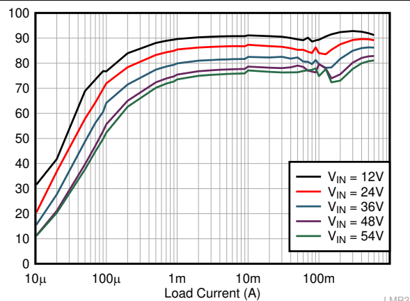
LMR36506R5 V_{OUT} = 5 V Fixed 1 MHz (AUTO)
