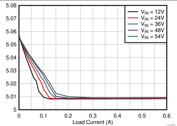
LMR36506R5 V_{OUT} = 5 V 1 MHz (AUTO)
