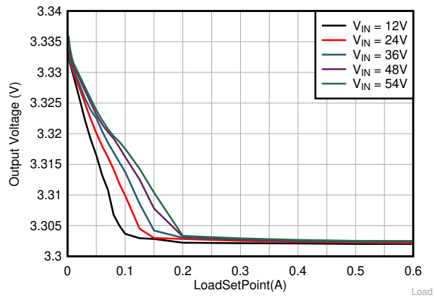
LMR36506R V_{OUT} = 3.3 V Fixed 1 MHz (AUTO)
