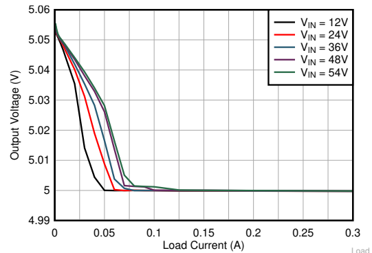
LMR36503R5 V_{OUT} = 5V Fixed 1 MHz (AUTO)
