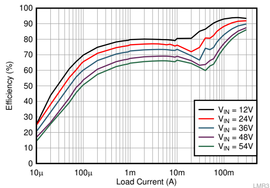
图 7-1. Efficiency 5-V Output, Auto Mode
