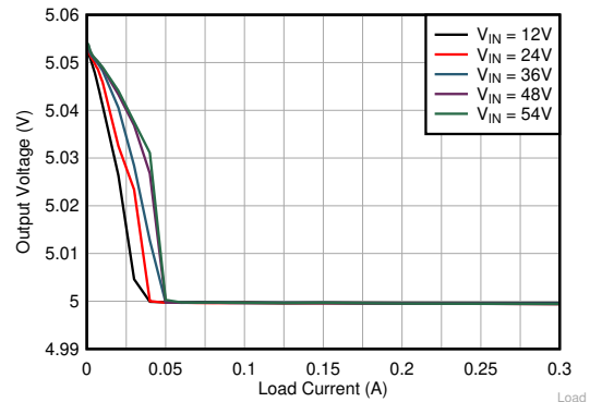
LMR36503R5 V_{OUT} = 5V Fixed 400 kHz (AUTO)
