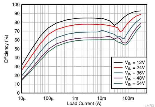
图 7-2. Efficiency 5-V Output, Auto Mode
