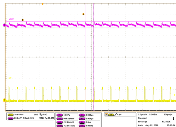
图 6-20. Steady State at 0-A Output Current
