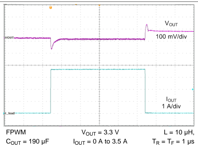
Figure 47. Load Transient
