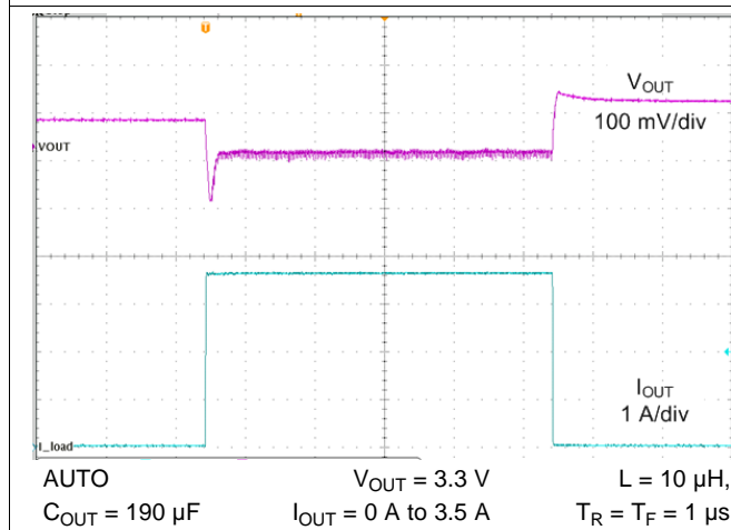
Figure 46. Load Transient
