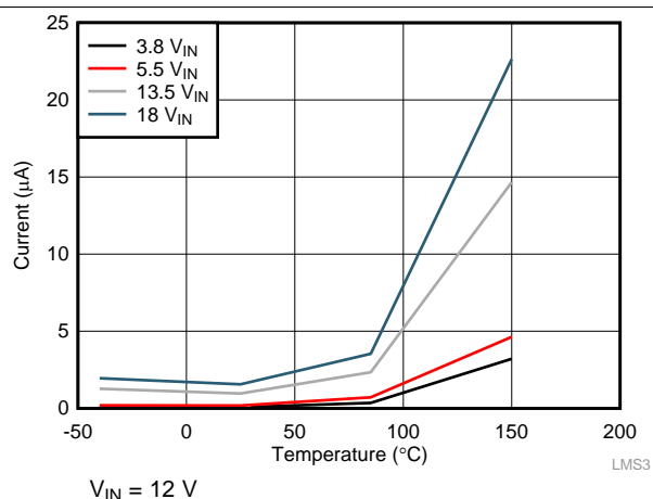
Figure 6. Shutdown Current
