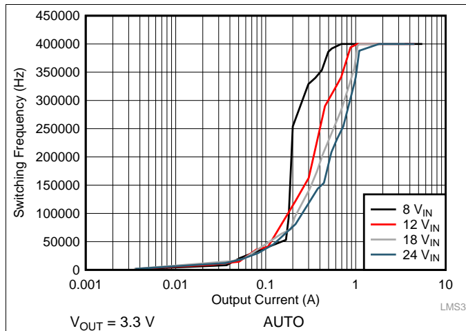
Figure 44. Switching Frequency vs Load Current
