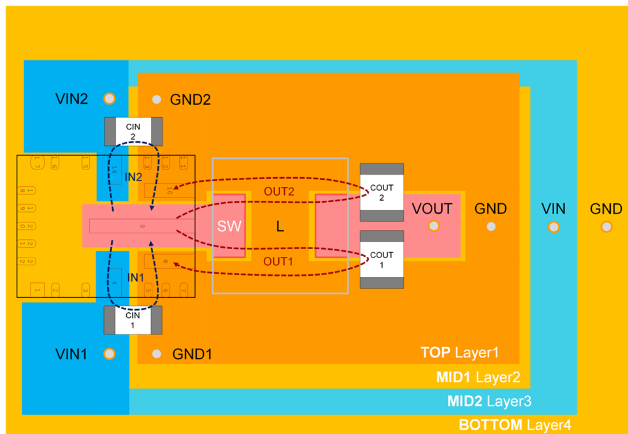
Figure 53. Layout of the Power Components and Current Flow
