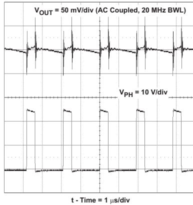
图 14. Output Voltage Ripple and PH Node
