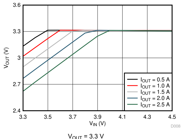
图 6-8. Dropout Curve
