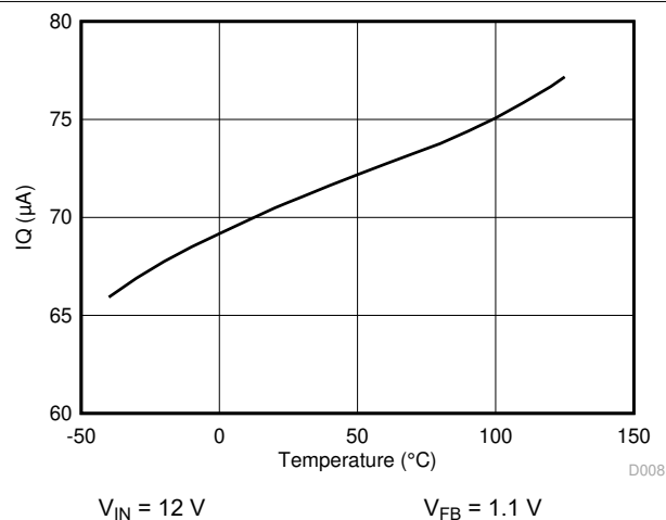
图 6-9. I_Q vs Junction Temperature
