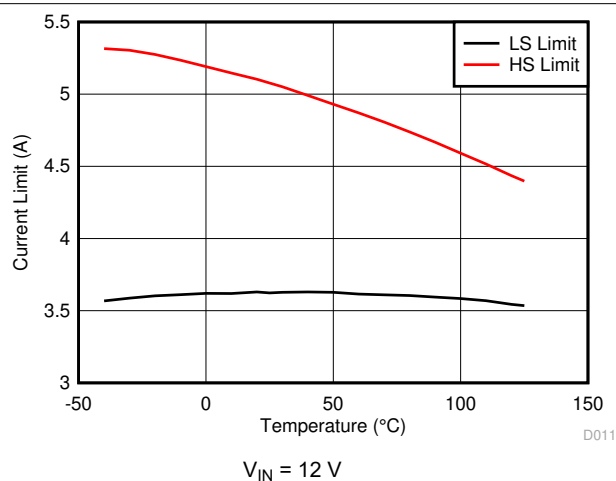
图 6-12. HS and LS Current Limit vs Junction Temperature
