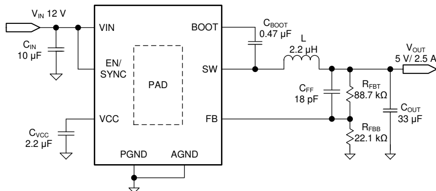
图 8-1. Application Circuit
