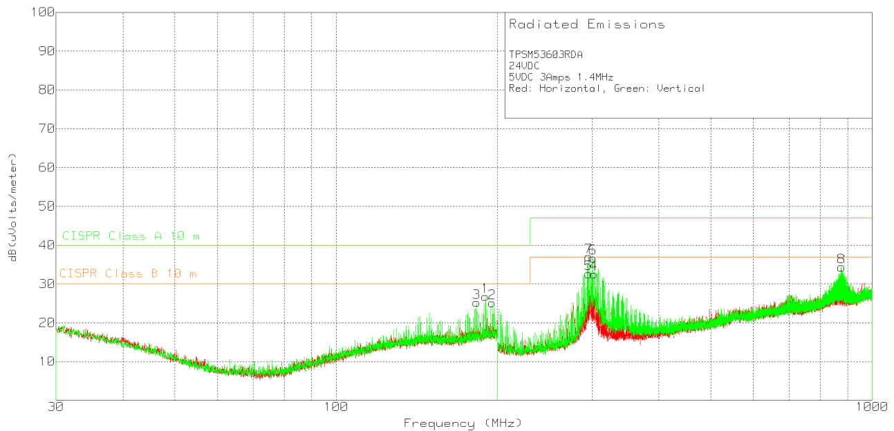
图 48. Radiated Emissions 24-V Input, 5-V Output, 3-A Load
