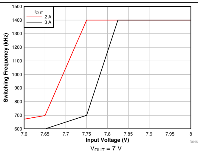
图 36. Frequency Foldback
