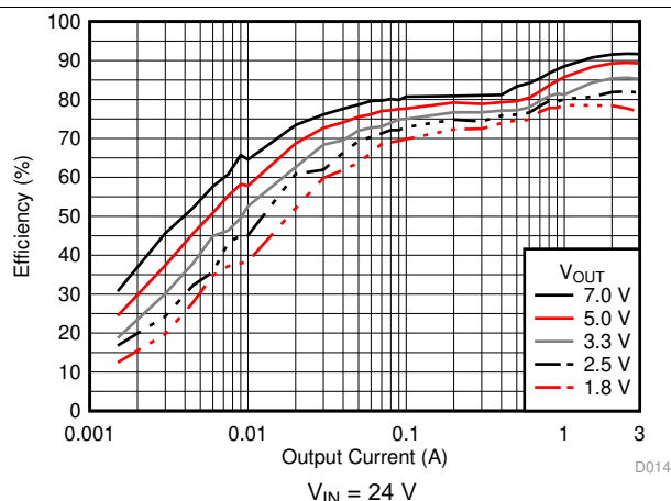
图 14. Efficiency versus Output Current
