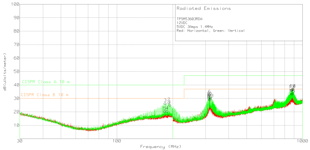
图 49. Radiated Emissions 12-V Input, 5-V Output, 3-A Load
