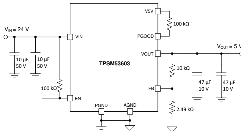
图 40. TPSM53603 Typical Schematic
