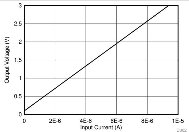
图 42. Photodiode Amplifier Circuit DC Results
