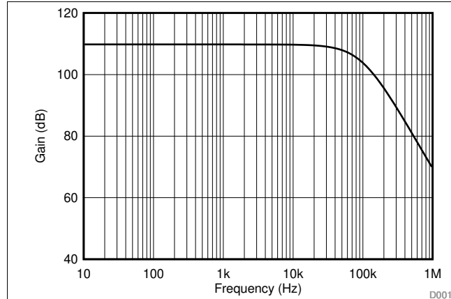
图 41. Photodiode Amplifier Circuit AC Gain Results
