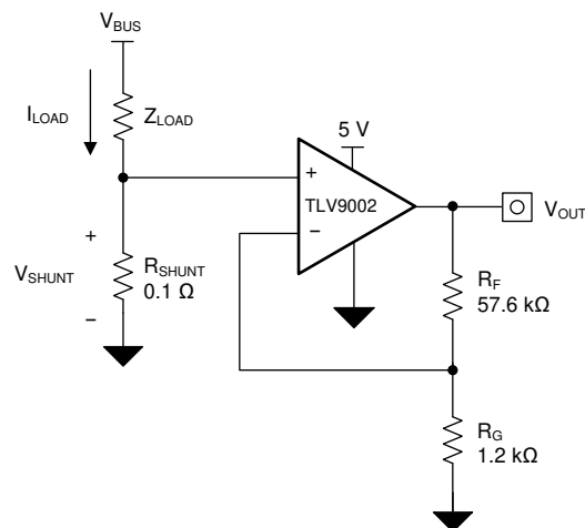
图 38. TLV900x in a Low-Side, Current-Sensing Application
