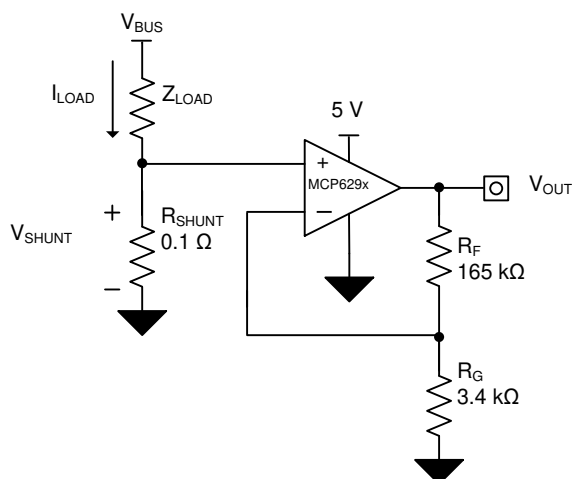
图 33. MCP629x in a Low-Side, Motor-Control Application
