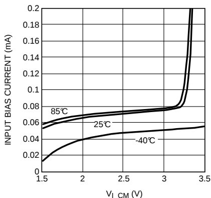
Figure 47. Input Bias Current vs Input CM
