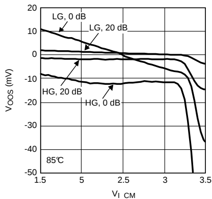
Figure 35. A_{V_{CM}}
