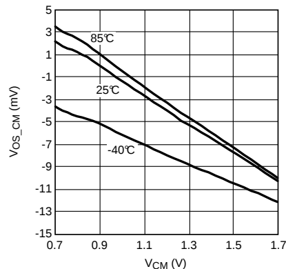
Figure 44. V_{OS\_CM} vs V_{CM}
