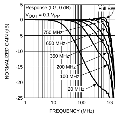
Figure 4. Small Signal Response (LG, 0 dB)
