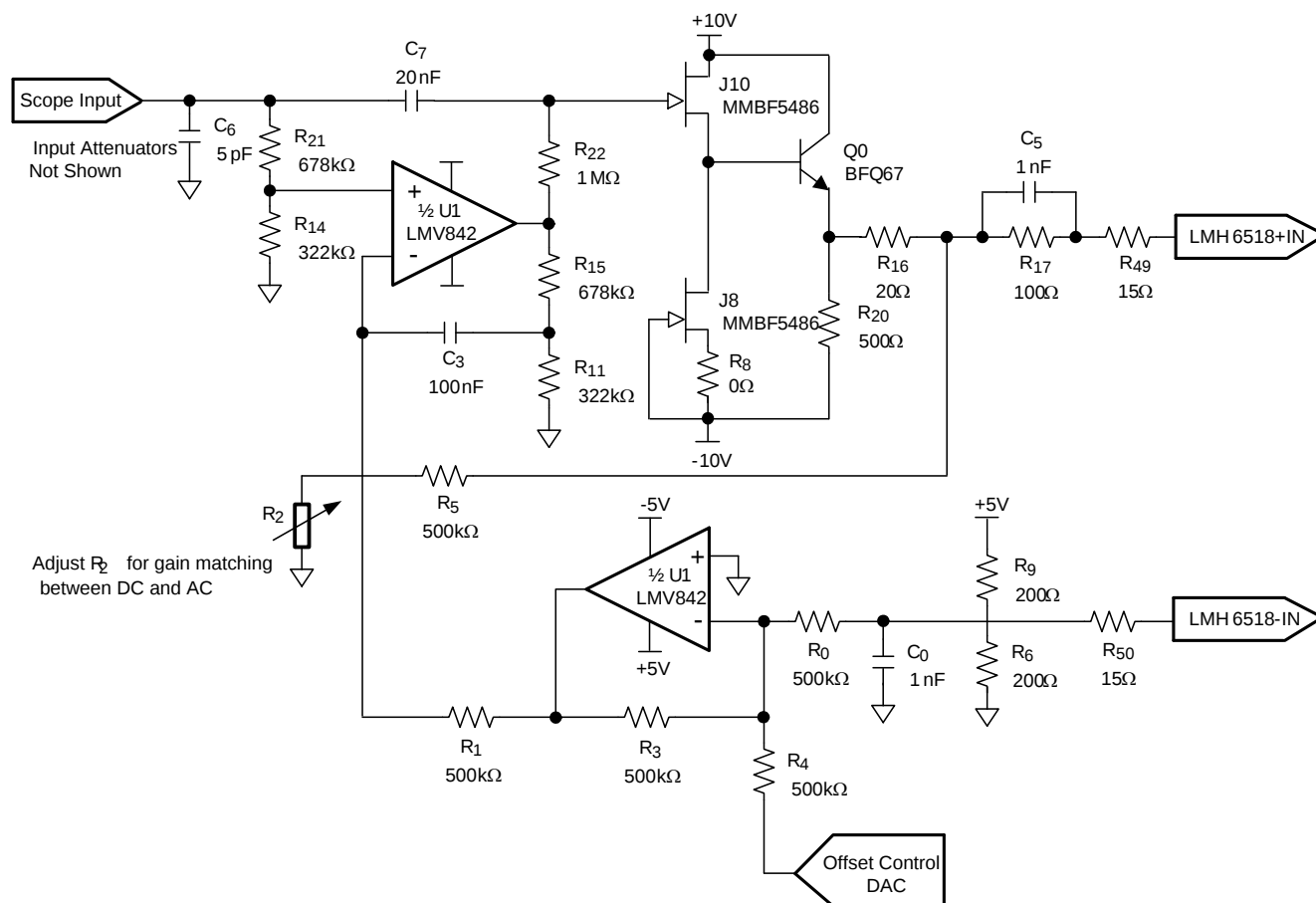
Figure 68. JFET LNA Implementation
