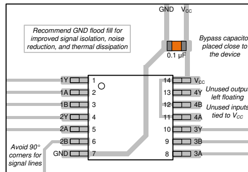
图 11. Example layout for the SN74HCS02
