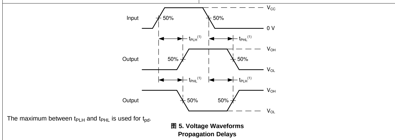
图 4. Voltage Waveforms Transition Times
