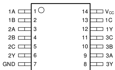
Figure 5-1. D, DB, N, NS, J, or W Package 14-Pin SOIC, SSOP, PDIP, SO, CDIP, or CFP Top View
