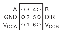
YZP Package 6-Pin DSBGA Bottom View
