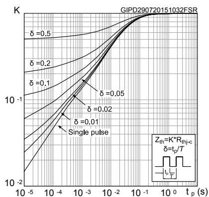
Figure 15. Thermal impedance
