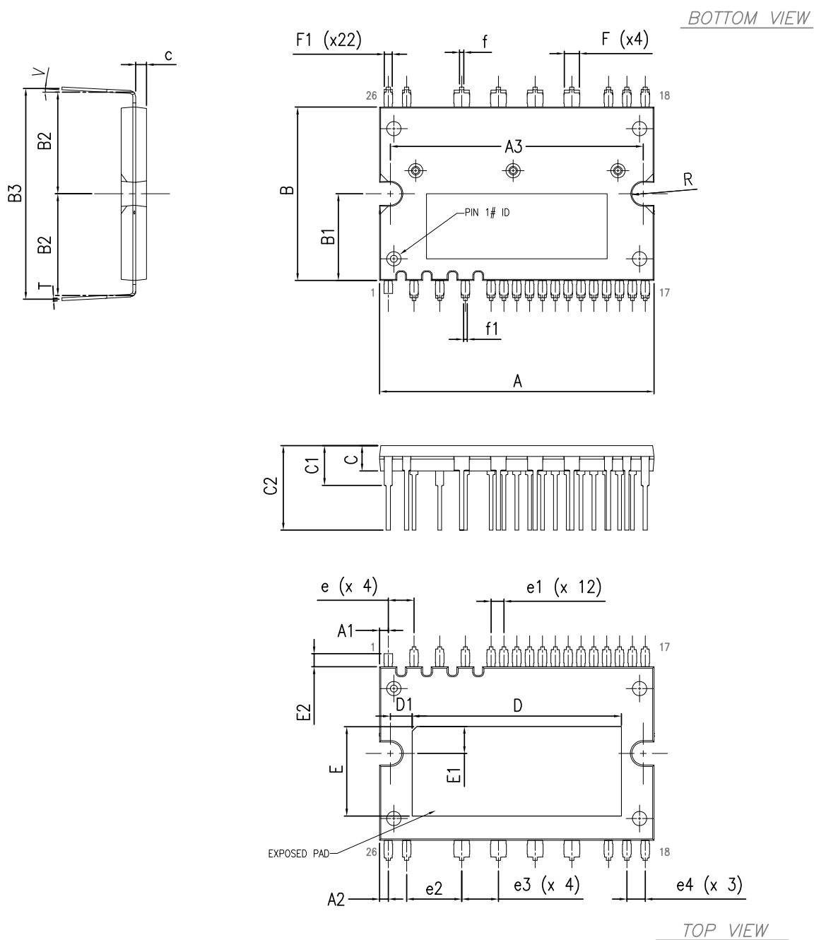
Figure 18. SDIP2B-26L type X package outline
