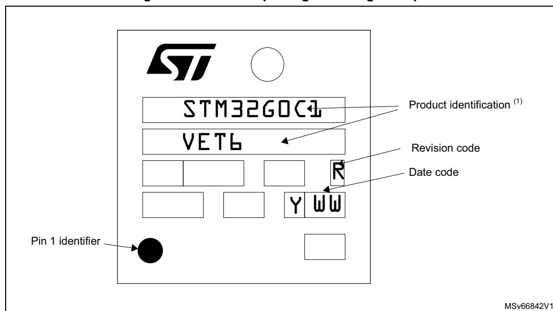
Figure 66. LQFP100 package marking example
