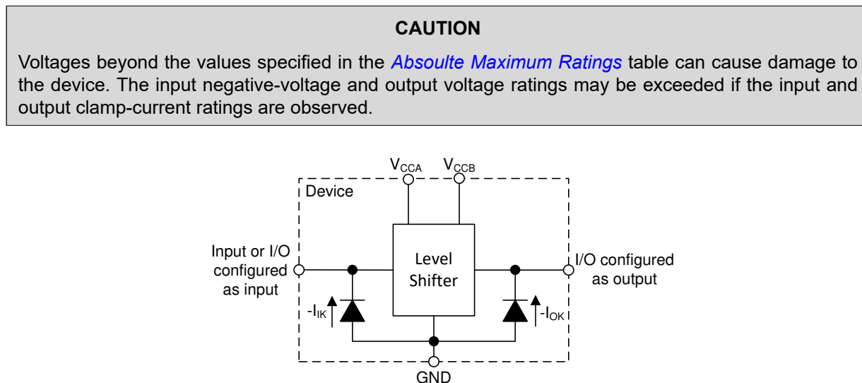
Figure 9-2. Electrical Placement of Clamping Diodes for Each Input and Output
