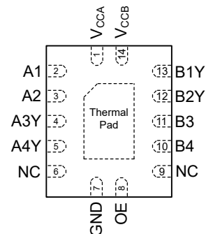
Figure 6-2. BQA Package Preview 14-Pin VQFN Top View
