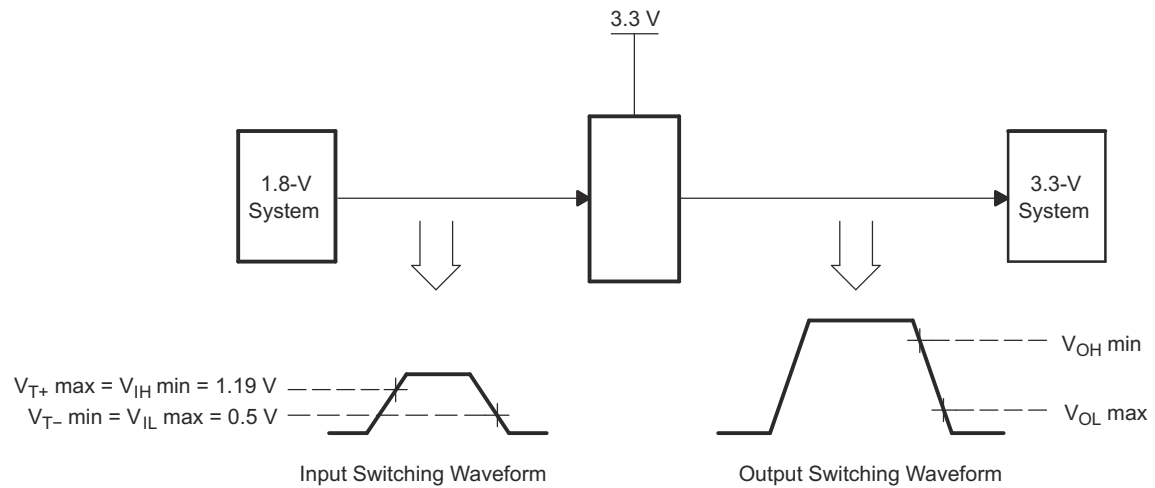
图 6-3. Switching Thresholds For 1.8-V To 3.3-V Translation
