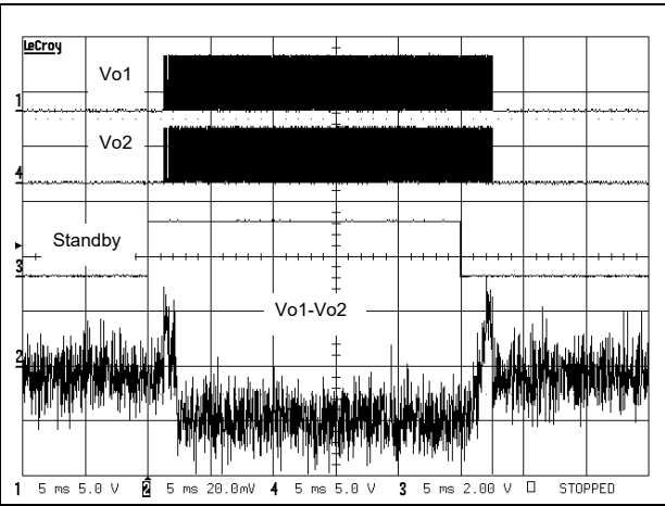
Figure 59. Startup & shutdown time V_{CC} = 5\text{ V} , G = 6\text{ dB} , No C_{in} (5 ms/div)
