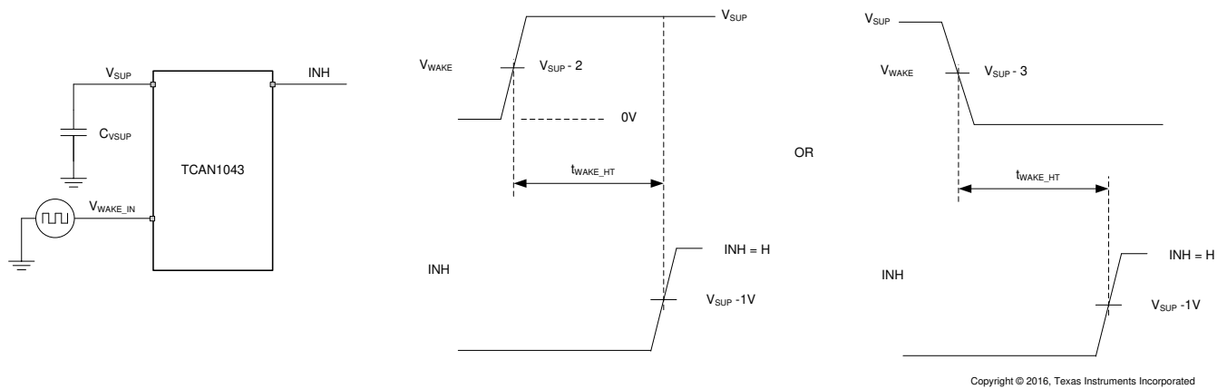
Figure 8-12. t_{Wake\_HT} While Monitoring INH Output
