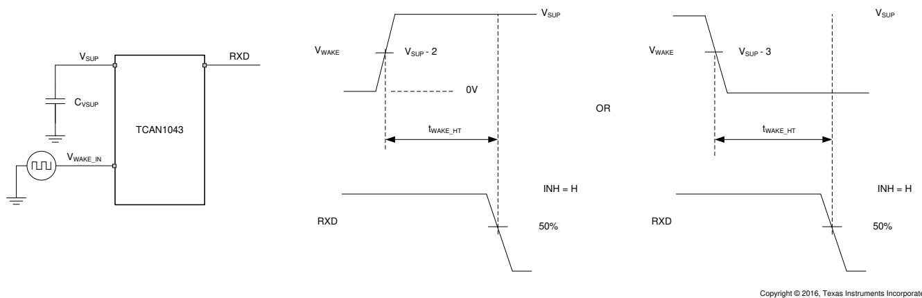
Figure 8-13. t_{Wake\_HT} While Monitoring RXD Output
