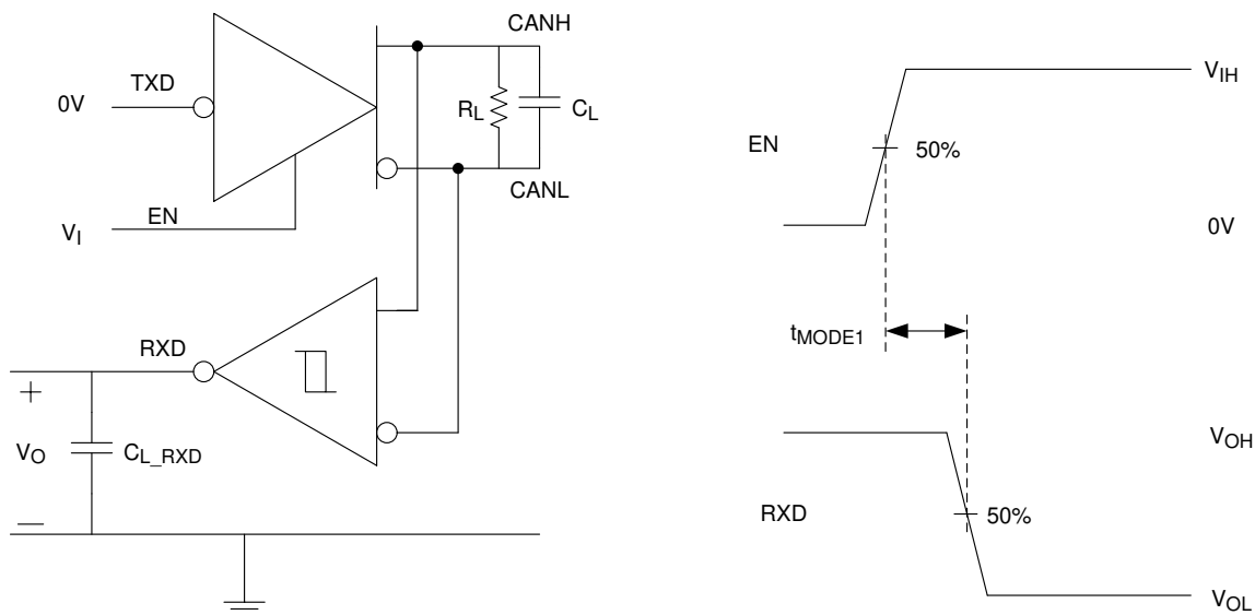
Figure 8-4. t_{\text{MODE1}} Test Circuit and Measurement, Silent Mode to Normal Mode
