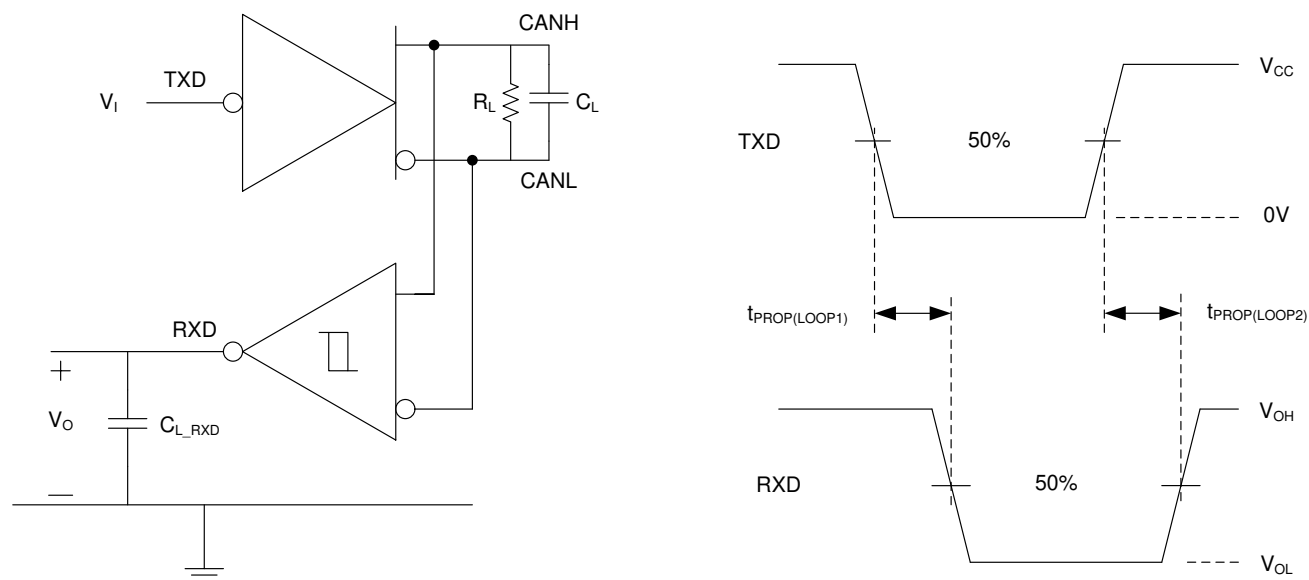
Figure 8-6. t_{\text{PROP(LOOP)}} Test Circuit and Measurement
