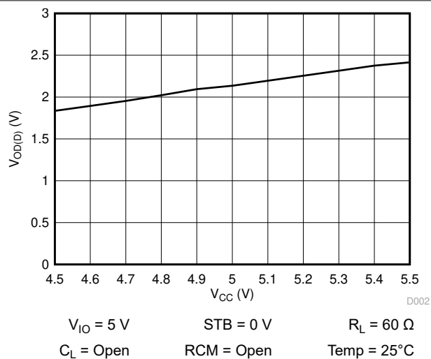
Figure 7-2. V_{OD(P)} over V_{CC}
