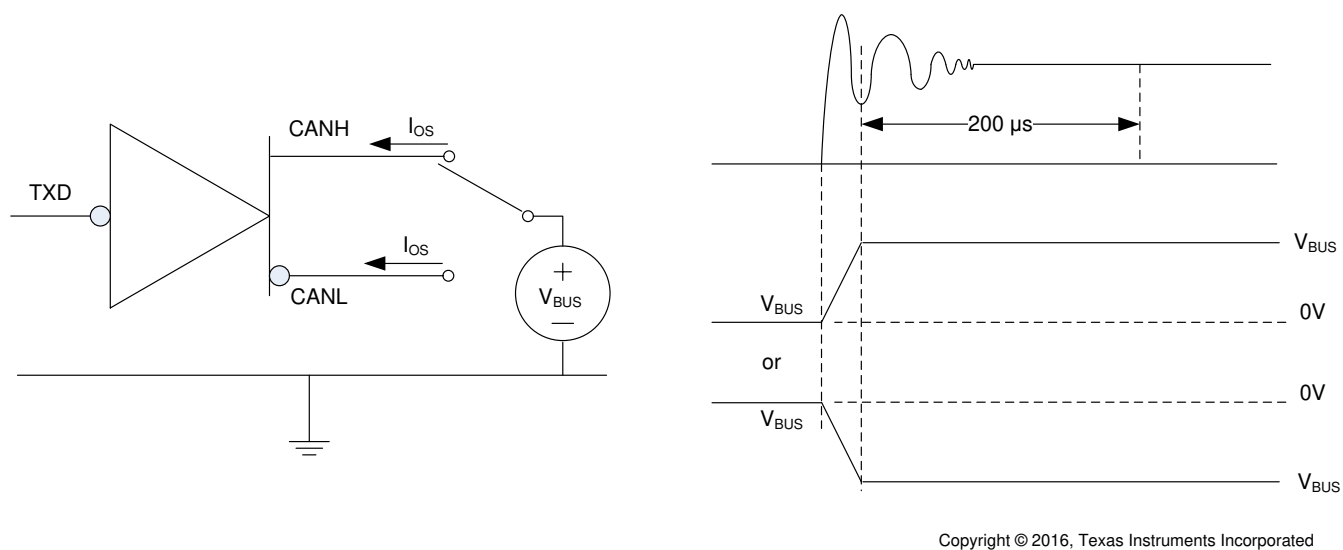
Figure 8-10. Driver Short-Circuit Current Test and Measurement
