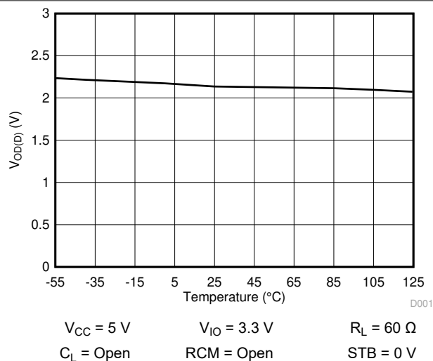
Figure 7-1. V_{OD(P)} over Temperature
