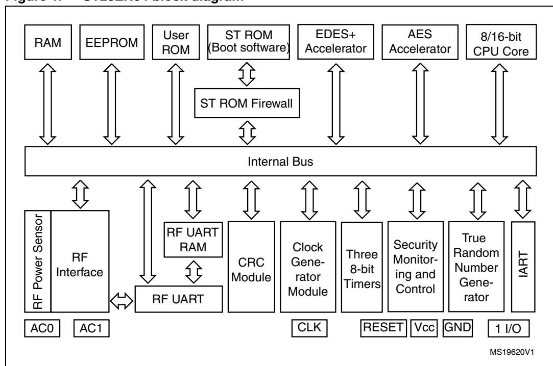
Figure 1. ST23ZR04 block diagram
