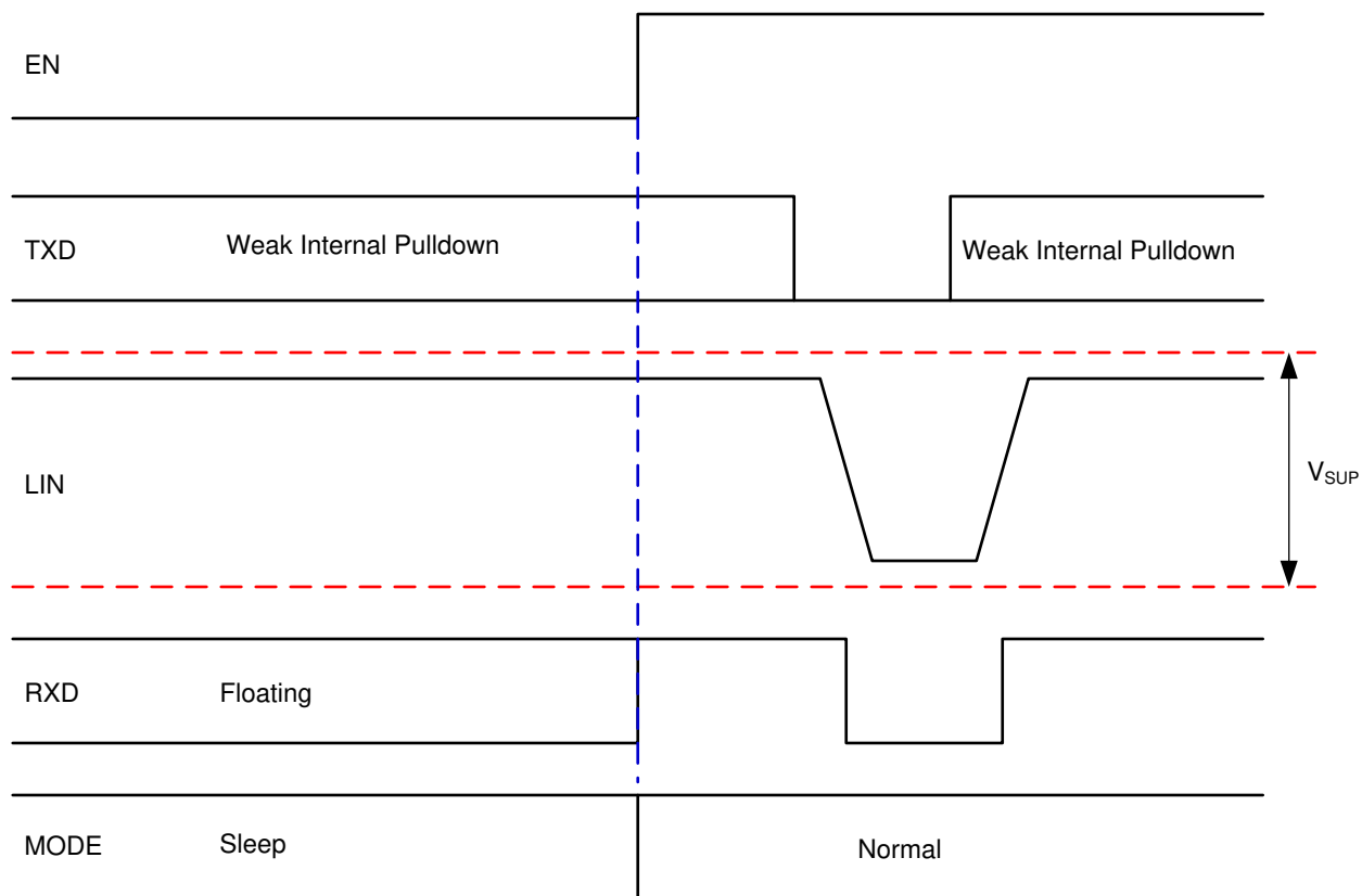
图 8-16. Wakeup Through EN
