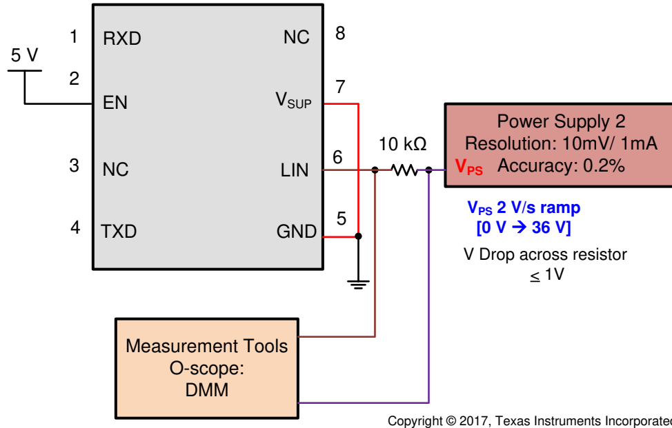
图 8-10. Test Circuit for I_{BUS\_NO\_BAT} Loss of Battery
