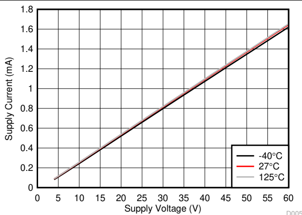
图 7-5. Standby Dominant I_{SUP} vs V_{SUP} and Temperature
