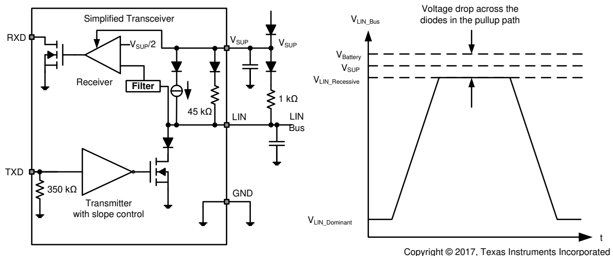
图 9-1. Leader Node Configuration with Voltage Levels
