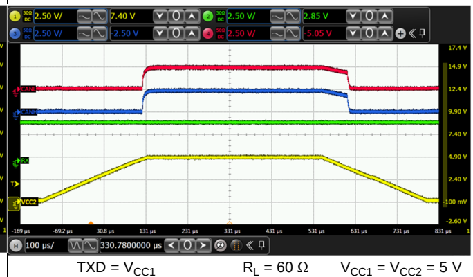
图 14. Glitch Free Power Up on V_{CC2} – CAN Bus Remains Recessive
