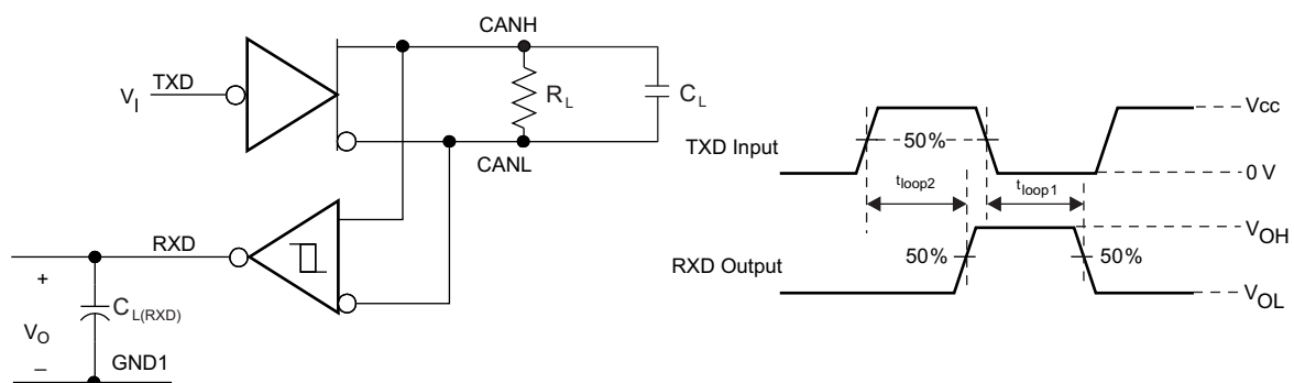
图 20. t_{\text{LOOP}} Test Circuit and Voltage Waveforms
