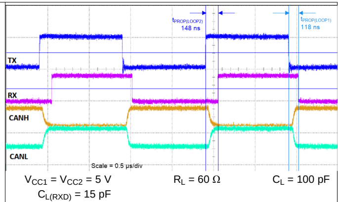
图 12. Typical TXD, RXD, CANH and CANL Waveforms at 1 Mbps
