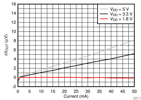
图 7-13. Injection Current vs Maximum Output Voltage shift
