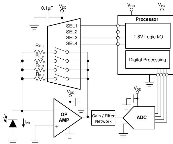
图 33. Switching Gain Settings of a TIA circuit
