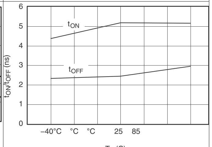
Figure 10. t_{ON} and t_{OFF} vs Temperature ( V_{CC} = 5V )
