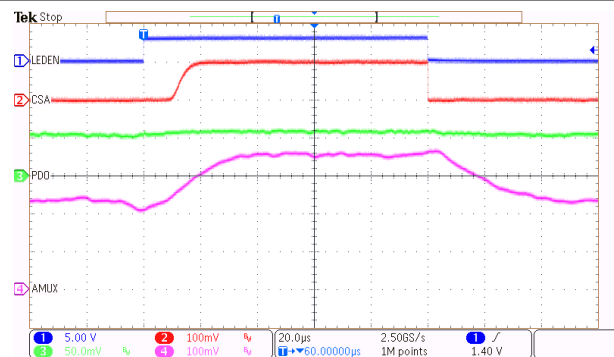
Figure 9-6. LED Driver and Photo Amplifier Waveforms
