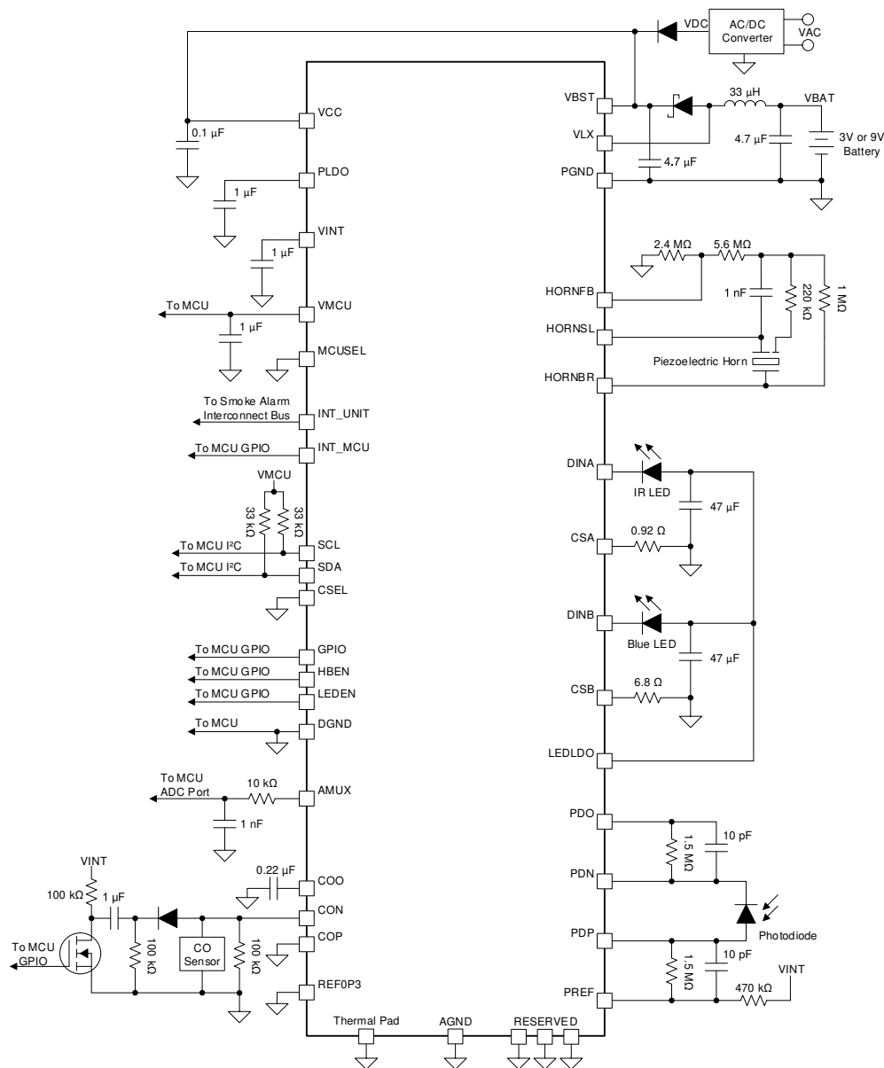
Figure 9-1. Dual-Wave Photoelectric Smoke and CO Alarm with Backup Battery
