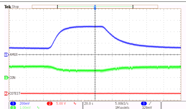
Figure 9-8. Carbon Monoxide Amplifier Waveforms with Calibration Gas
