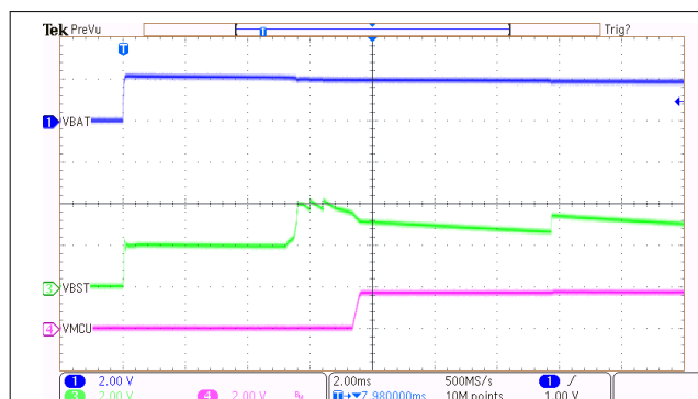
Figure 9-2. Power-up Waveforms
