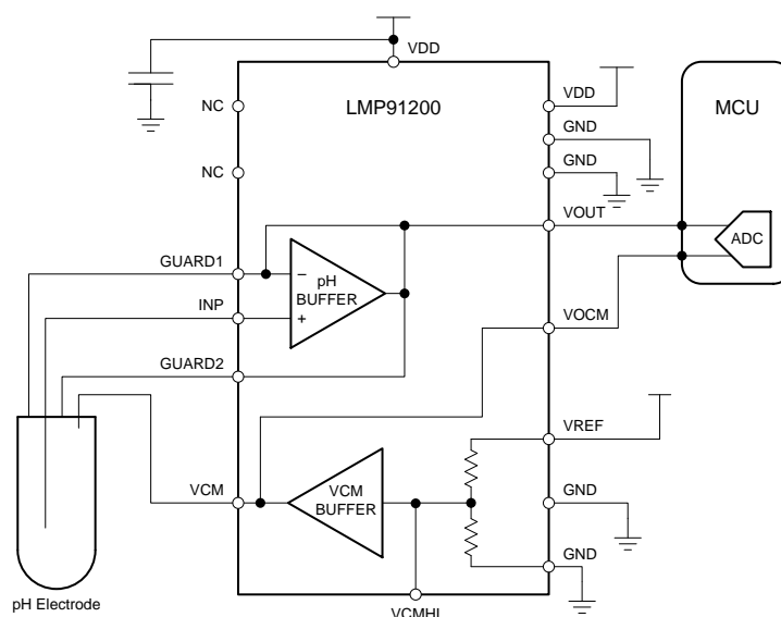
Figure 34. Typical Application
