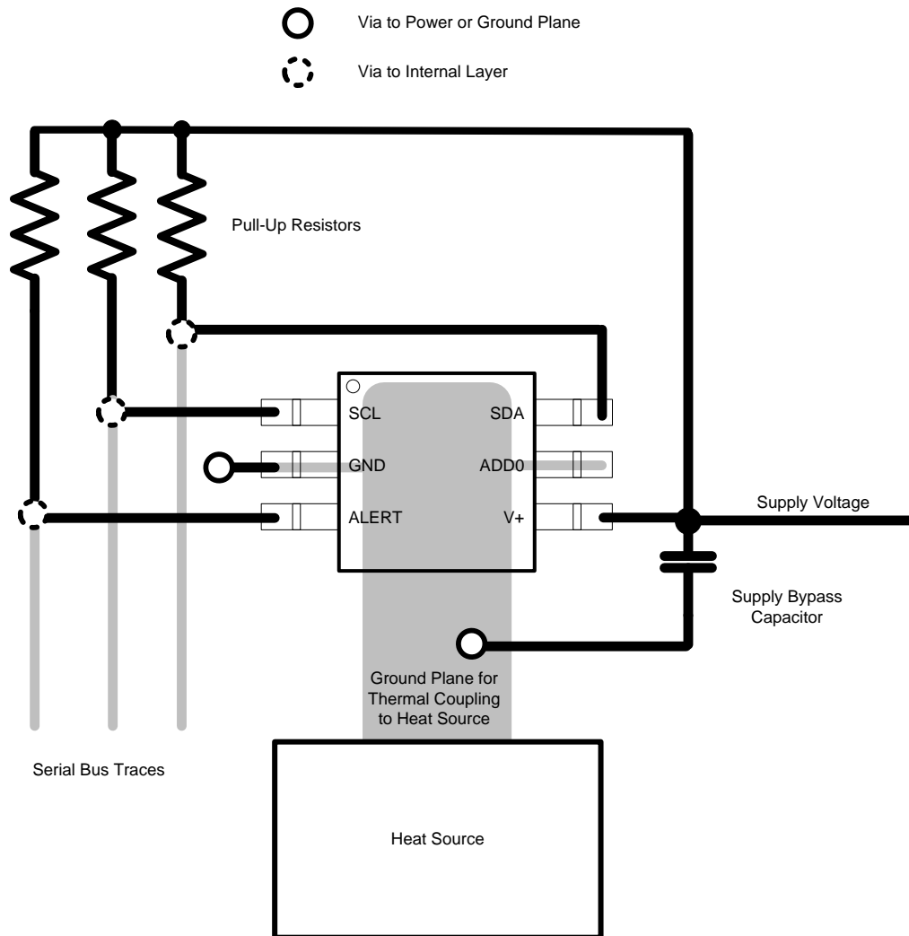
Figure 16. TMP101-Q1 Layout Example
