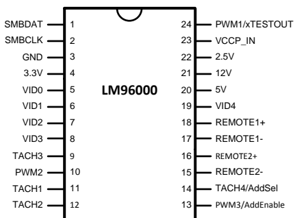
Figure 1. 24-Pin TSSOP Package
