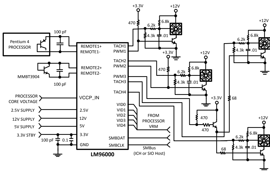
Figure 11. Typical Applications Schematic
