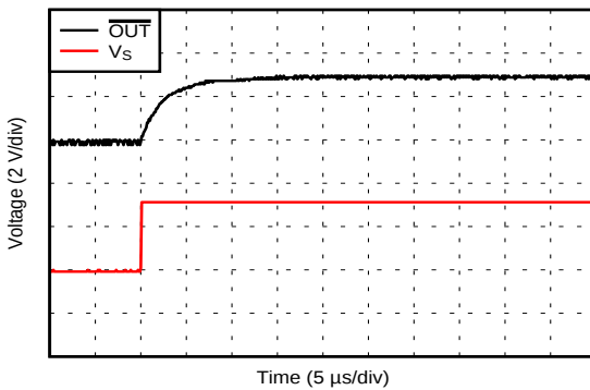
Figure 12. TMP302A Power-On Response, T_A Less than 50°C
