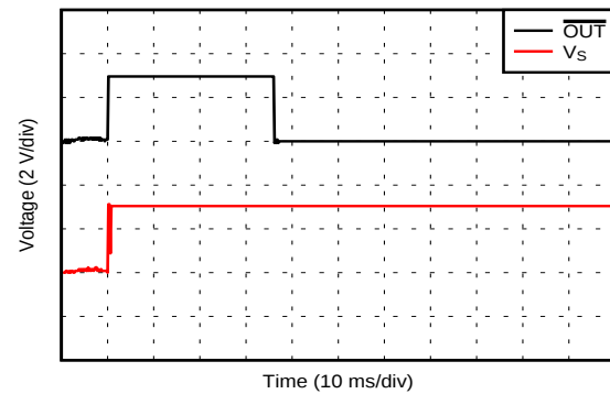
Figure 13. TMP302A Power-On Response, T_A Greater than 50°C
