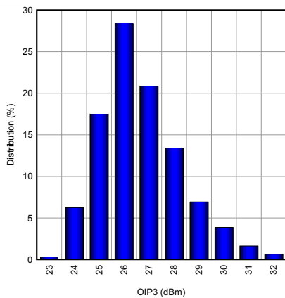
Figure 92. OIP3 at 2300-MHz Distribution
