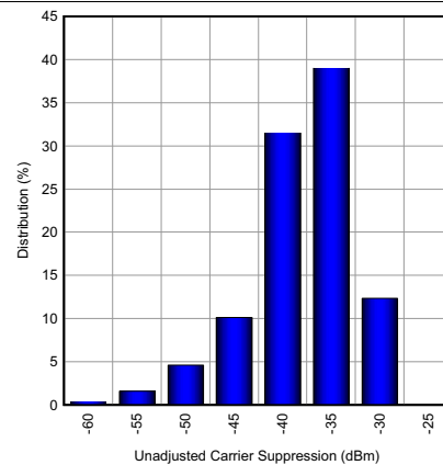
Figure 93. Unadjusted Carrier Suppression at 2300-MHz Distribution
