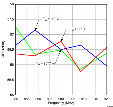
Figure 59. OIP2 vs Frequency and Temperature at 900 MHz
