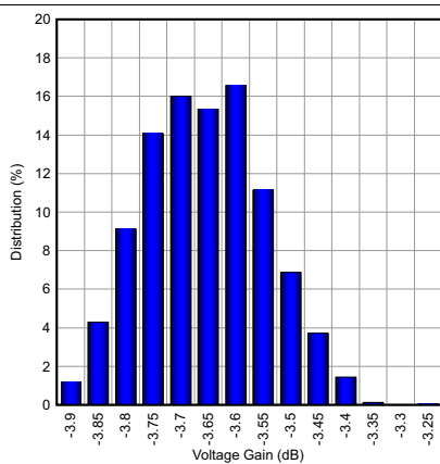
Figure 90. Gain at 2300-MHz Distribution
