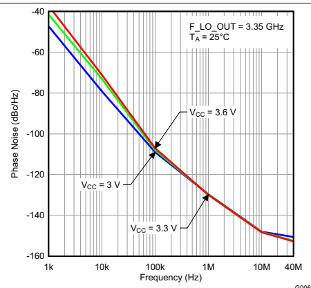
Figure 8. Open Loop Phase Noise vs Frequency and Supply Voltage
