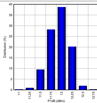
Figure 91. P1dB at 2300-MHz Distribution
