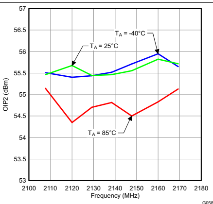
Figure 61. OIP2 vs Frequency and Temperature at 2150 MHz
