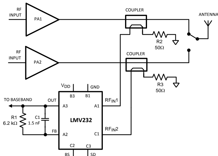
Figure 21. Typical Application
